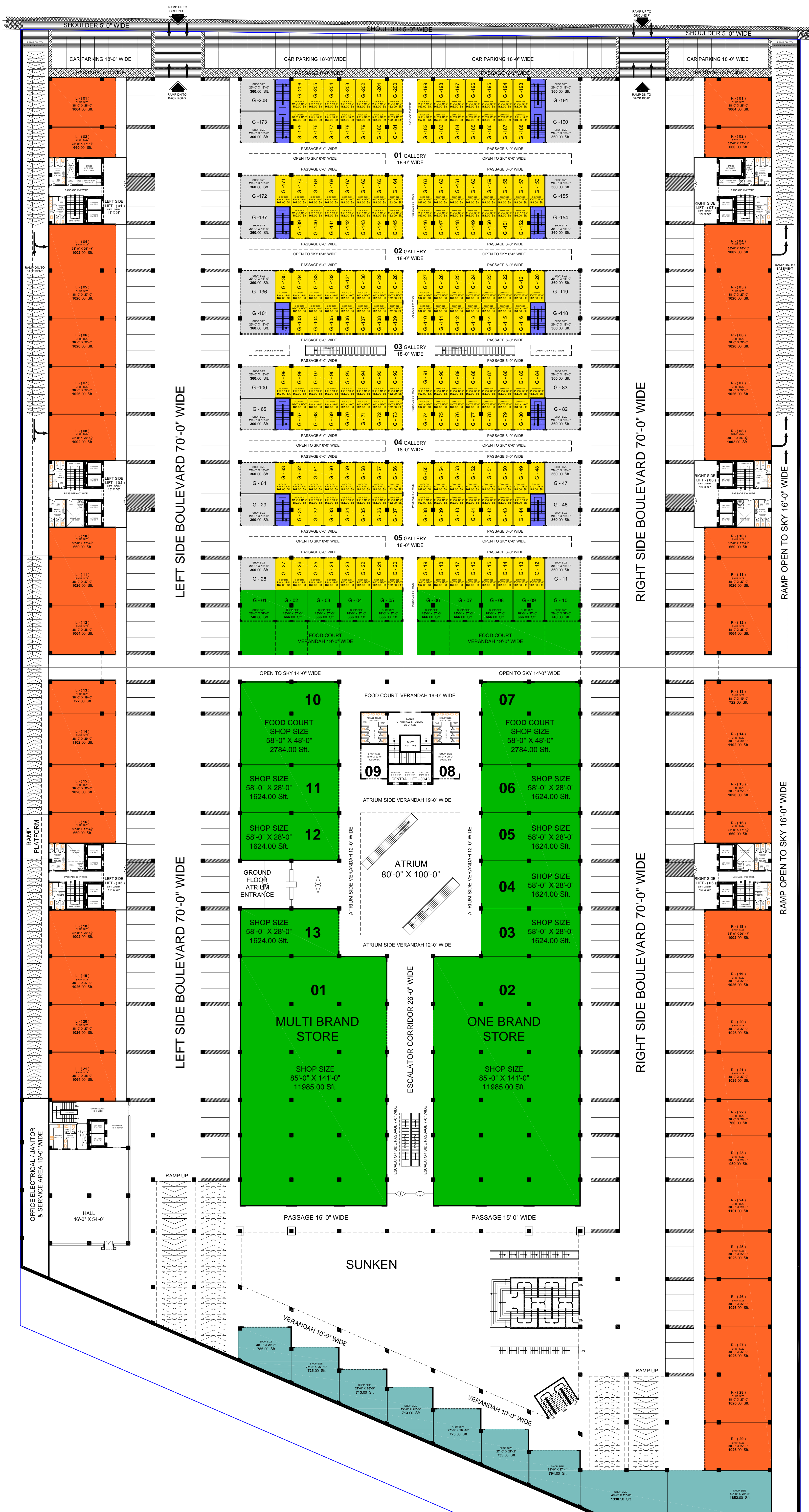
GROUND FLOOR PLAN ROYAL MALL SHOPPING FLOOR SOUK SHOPPING FLOOR
